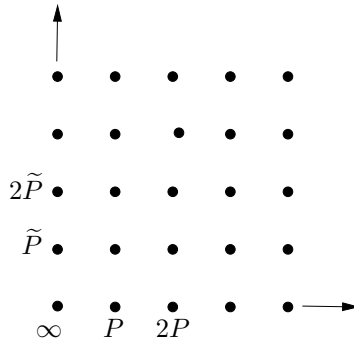
Figure 3: N^2 points of order dividing N in E(\mathbb{F}_{p^2}) . The horizontal axis is in E(\mathbb{F}_p) .
