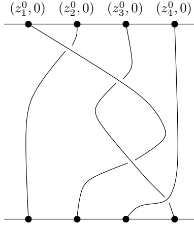
Figure 5: A geometric braid for n = 4 .
